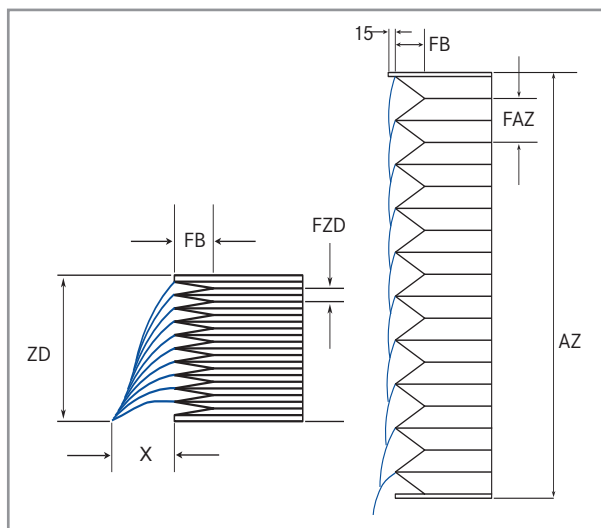
Drawing of FASTAM
